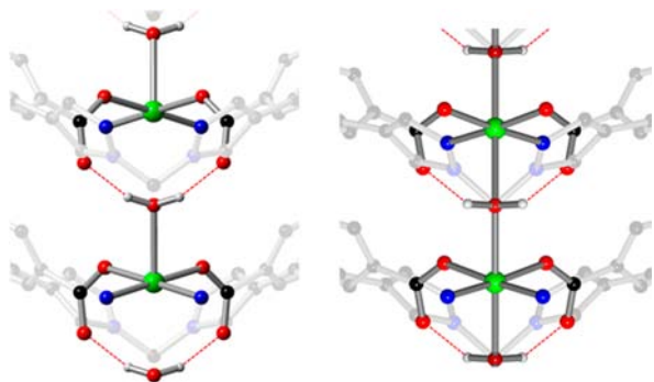
Figure 2. Enlargements of the hydrogen bonding in (left) [Cu( bcppm )H 2 O]·xS (between the 2D layers) and (right) [Cu( bcppm )H 2 O]·heated.
