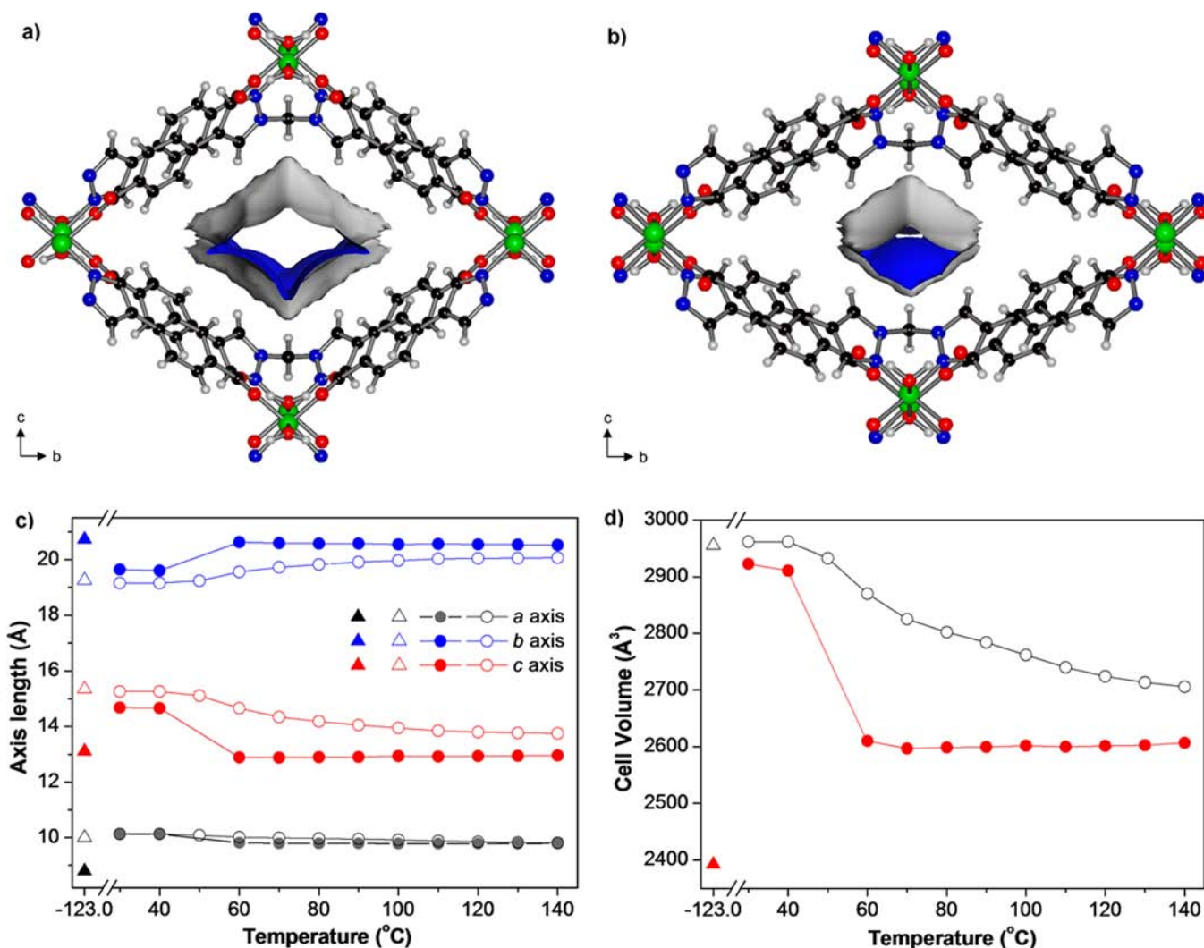
Figure 4. Representations of the crystal structures of (a) [Cu(bcppm)H 2 O]·xS and (b) [Cu(bcppm)H 2 O]-heated showing the solvent-accessible pore surface with a probe of diameter 3.30 Å. Color - Cu, green; C, Black; N, Blue; O, Red; H, Grey. (c) Temperature-dependent changes of the unit cell axes determined from indexing the PXRD data: open circles, [Cu(bcppm)H 2 O]·xS; filled circles, [Cu(bcppm)H 2 O]-acetone. Open and filled triangles represent the unit cell dimensions from the crystal structures of [Cu(bcppm)H 2 O]·xS and [Cu(bcppm)H 2 O]-heated, respectively. (d) Temperature-dependent changes of the unit cell volume: open black circles, [Cu(bcppm)H 2 O]·xS; red circles, [Cu(bcppm)H 2 O]-acetone; black triangle, cell volume from the crystal structure of [Cu(bcppm)H 2 O]·xS; red triangle, cell volume of [Cu(bcppm)H 2 O]-heated.
