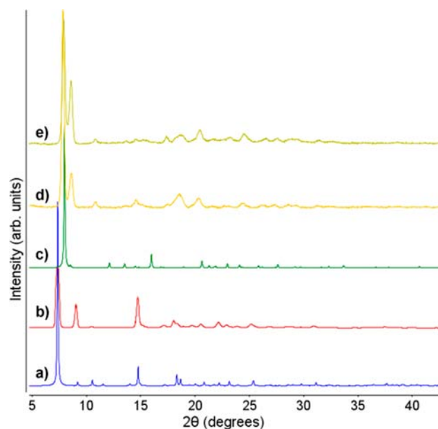
Figure 3. PXRD patterns of (a) [Cu( bcppm )H 2 O]·xS (blue, simulated); (b) [Cu( bcppm )H 2 O]·xS (red); (c) [Cu( bcppm )H 2 O]·heated (green, simulated); (d) [Cu( bcppm )H 2 O]-ac (yellow); and (e) [Cu( bcppm )H 2 O]-ac exposed to 1 bar of CO 2 (khaki).
