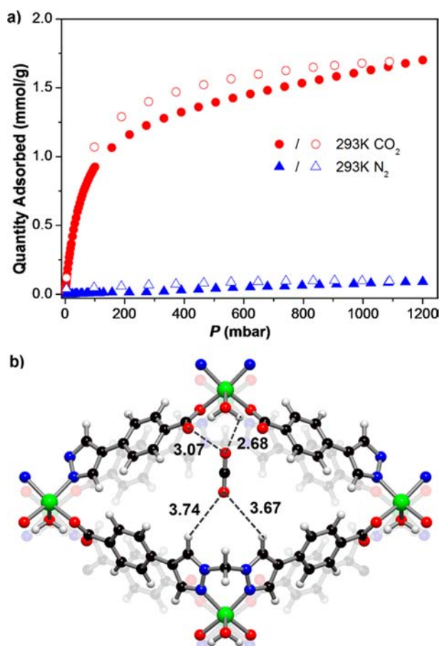
Figure 5. (a) CO 2 and N 2 isotherms at 293 K. (b) A view showing the location of CO 2 in [Cu(bcppm)H 2 O]-ac identified from NVT-simulated annealing. Selected distances between the CO 2 molecule and the framework atoms are shown in angstroms.
