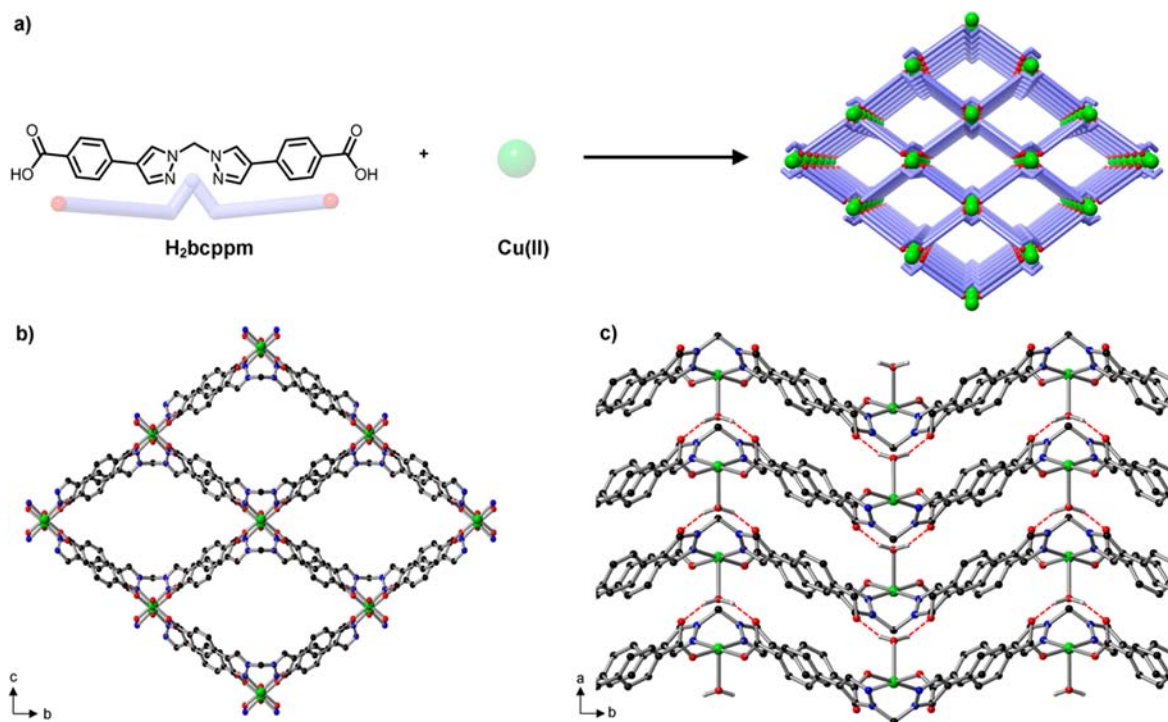
Figure 1. (a) Schematic representation of the synthesis of [\text{Cu}(\text{bcppm})\text{H}_2\text{O}]\cdot x\text{S} showing a simplified representation of the structure. (b) View of the pores of [\text{Cu}(\text{bcppm})\text{H}_2\text{O}]\cdot x\text{S} along the a -axis, and (c) view along the c -axis.
